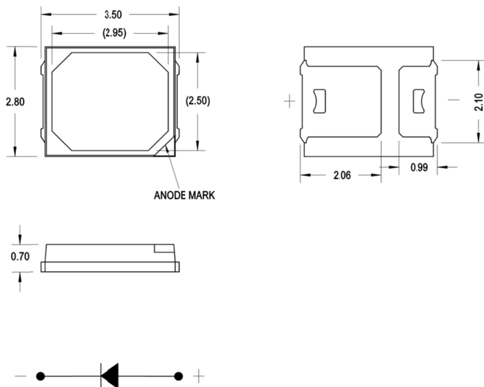
Figure 1: Package Drawing
