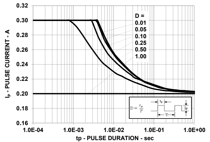
Figure 14: Pulse Handling Capability at T_s \leq 100^{\circ}\text{C} (Far Red)
